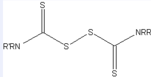
Thiram Disulphides
