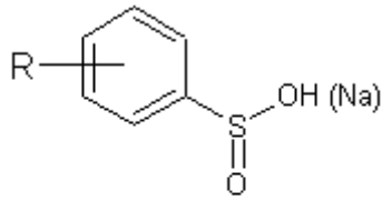
Sulphinic acid / Sodium sulphininate
