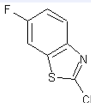
2-Chloro-6-fluorobenzothiazole
