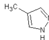
4-Methylpyrazole
