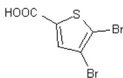
2,3-Dibromothiophene-5-carboxylic acid
