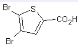
2,3-Dibromothiophene-5-carboxylic acid
