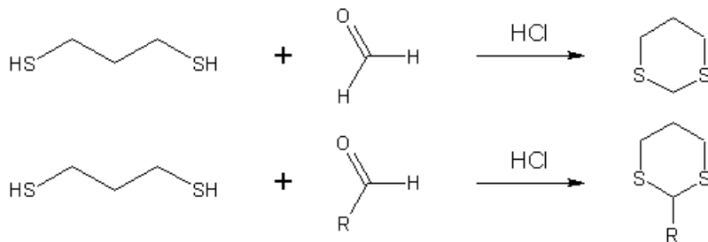
Propane-1,3-dithiol
