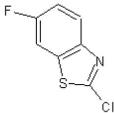
2-Chloro-6-fluorobenzothiazole
