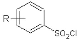
Sulphonyl chlorides
