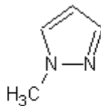
N-Methyl pyrazole
