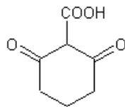
1,3-Cyclohexanedione-2-carboxylic acid
