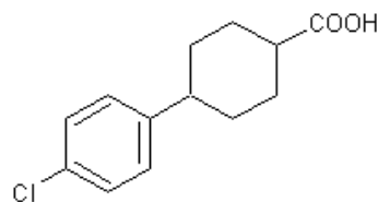
4-(p-Chlorophenyl)-1-cyclohexanecarboxylic acid
