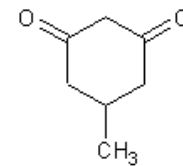
5-Methyl-1,3-Cyclohexanedione
