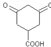
1,3-Cyclohexanedione-5-carboxylic acid
