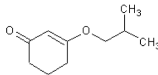
3-Isobutoxy-2-cyclohexen-1-one
