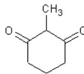
2-Methyl-1,3-Cyclohexanedione
