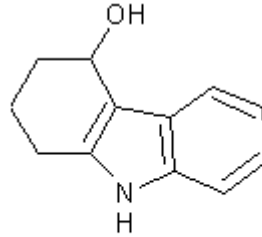
4-Hydroxycarbazole
