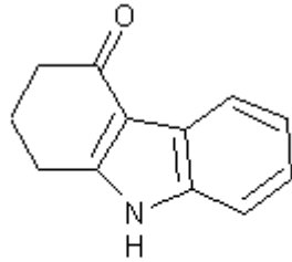
Tetrahydro-4-oxocarbazole
