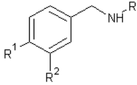
substituted Benzylamines
