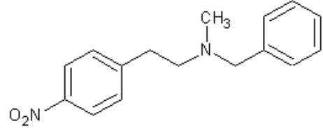
N-benzyl protected Amines
