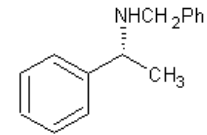
(R)-(+)-N-Benzyl- \alpha -phenethylamine
