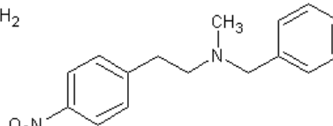
N-Benzyl protected amines
